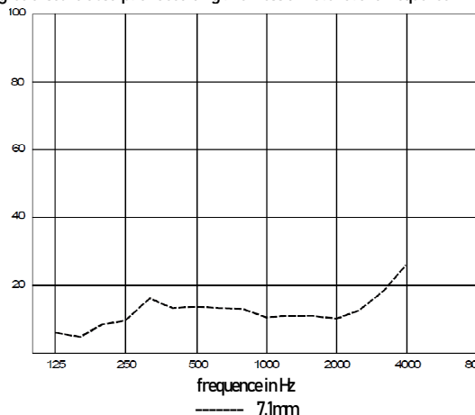
Degree of sound absorption according thickness of material and frequency DIN 52215
