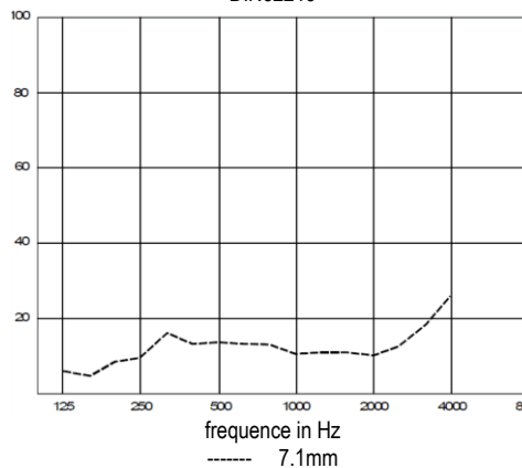
Degree of sound absorption according thickness of material and frequency DIN52215
